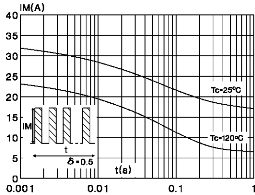
Fig.6 : Non repetitive surge peak forward current versus overload duration. (Maximum values) (ISOWATT220AB) (Per diode)
